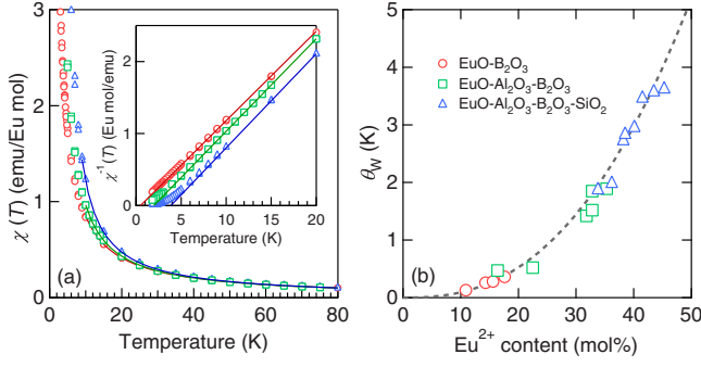
FIG. 3. (Color online) (a) Temperature dependence of magnetic susceptibility, \chi(T) , of 30.0EuO·70.0B 2 O 3 (30EuB2, red circle), 52.5EuO·10.0Al 2 O 3 ·37.5B 2 O 3 (53EuAIB, green square), and 60.0EuO·11.0Al 2 O 3 ·19.5B 2 O 3 ·9.5SiO 2 (60EuAIBSi, blue triangle) glasses. The solid curve represents the fit of Eq. (1) to the experimental data. The inset shows temperature dependence of inverse magnetic susceptibility, \chi^{-1}(T) , of the present glasses. The solid lines in the inset represent the fit of Curie-Weiss law to the experimental data in high-temperature region. (b) The Weiss temperature, \theta_W , is plotted against the concentration of Eu 2+ ion. The dashed curve is a guide to eyes.
