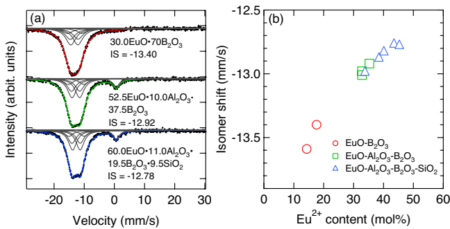
FIG. 2. (Color online) (a) ^{151}\text{Eu} Mössbauer spectra of 30.0\text{EuO}\cdot 70.0\text{B}_2\text{O}_3 (30EuB2), 52.5\text{EuO}\cdot 10.0\text{Al}_2\text{O}_3\cdot 37.5\text{B}_2\text{O}_3 (53EuAIB), and 60.0\text{EuO}\cdot 11.0\text{Al}_2\text{O}_3\cdot 19.5\text{B}_2\text{O}_3\cdot 9.5\text{SiO}_2 (60EuAIBSi) glasses at room temperature. The values of IS are also shown. The calculated spectra are drawn as solid curves. (b) Relationship between the IS value and \text{Eu}^{2+} concentration: 25EuB2, 30EuB2 (red open circles), 50EuAIB3, 50EuAIB4, 53EuAIB (green open squares), 47EuAIBSi, 55EuAIBSi, 58EuAIBSi2, 59EuAIBSi, and 60EuAIBSi (blue open triangle). For the abbreviation of notation, see Table I.
