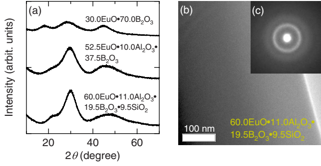
FIG. 1. (Color online) (a) XRD patterns of 30.0\text{EuO}\cdot 70.0\text{B}_2\text{O}_3 (30EuB2), 52.5\text{EuO}\cdot 10.0\text{Al}_2\text{O}_3\cdot 37.5\text{B}_2\text{O}_3 (53EuAIB), and 60.0\text{EuO}\cdot 11.0\text{Al}_2\text{O}_3\cdot 19.5\text{B}_2\text{O}_3\cdot 9.5\text{SiO}_2 (60EuAIBSi) glasses. (b) TEM image and (c) SAED of 60.0\text{EuO}\cdot 11.0\text{Al}_2\text{O}_3\cdot 19.5\text{B}_2\text{O}_3\cdot 9.5\text{SiO}_2 glass.
